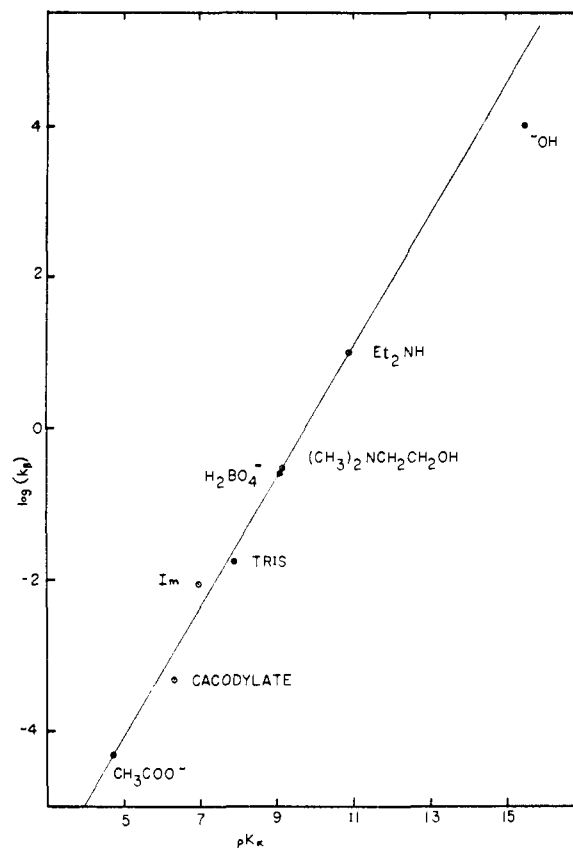
Figure 2. Bronsted plot of \log k_{13} vs. the \text{p}K_a of the catalyzing base in the cyclization of ethyl 2-hydroxymethylbenzoate to phthalide at 30^\circ in \text{H}_2\text{O} ( \mu = 0.5 ).
